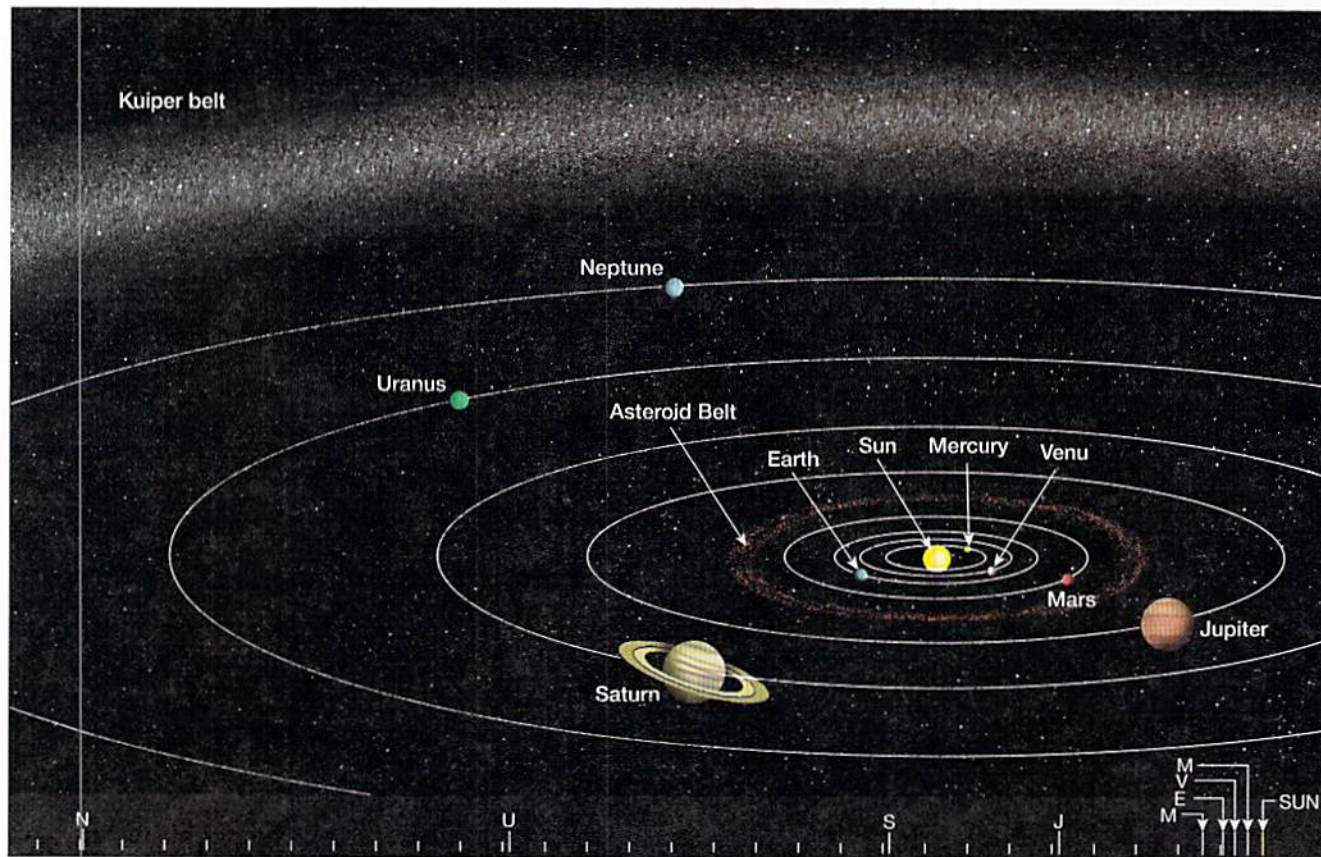
FIGURE 22.1 Orbits of the planets. Positions of the planets are shown to scale along bottom of diagram.
