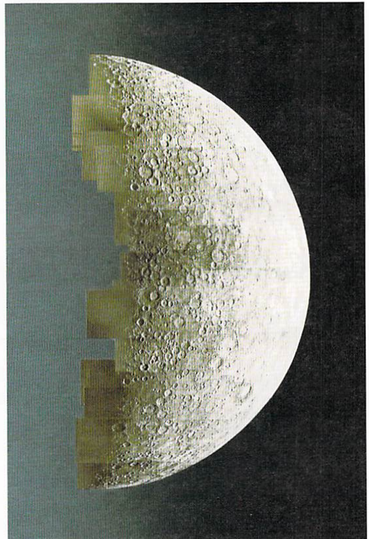
FIGURE 22.10 Photomosaic of Mercury. This view of Mercury is remarkably similar in appearance to the "far side" of Earth's Moon. (NASA)
