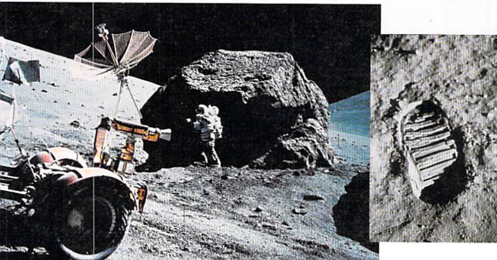
FIGURE 22.8 Astronaut Harrison Schmitt sampling the lunar surface. Notice the footprint (inset) in the lunar "soil." (NASA)
