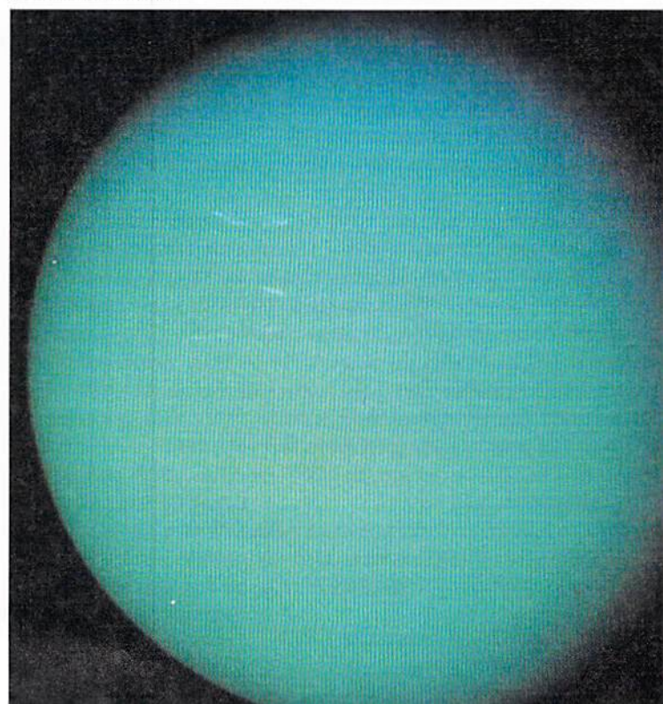
FIGURE 22.23 This image of Uranus was sent back to Earth by Voyager 2 as it passed by this planet on January 24, 1986. Taken from a distance of nearly 1 million kilometers (620,000 miles), little detail of its atmosphere is visible, except for a few streaks (clouds) in the northern hemisphere (Courtesy of NASA)
