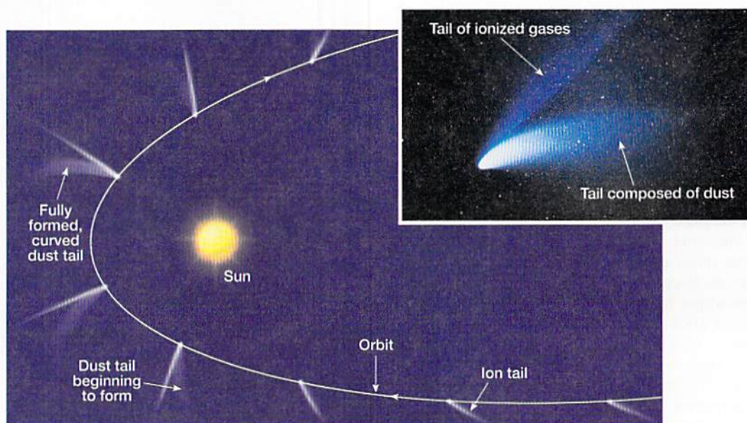
FIGURE 22.27 Orientation of a comet's tail as it orbits the Sun. Inset photo shows comet Hale-Bopp. The two tails seen in the photograph are between 10 million and 15 million miles long. (Peoria Astronomical Society photograph by Eric Clifton and Craig Neaveill)
