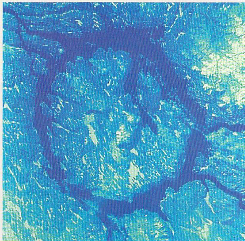
FIGURE 22.C Manicouagan, Quebec, is a 200-million-year-old eroded impact structure. The lake outlines the crater remnant, which is 70 kilometers (42 miles) across. Fractures related to this event extend outward for an additional 30 kilometers. (Courtesy of U.S. Geological Survey)
