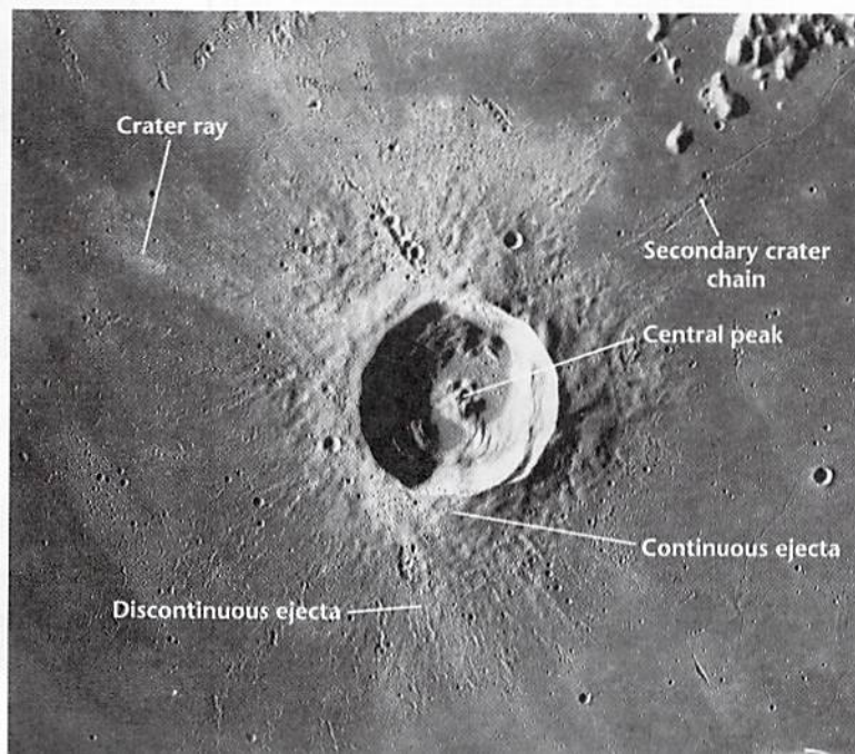
FIGURE 22.5 The 20-kilometer-wide (12-mile-wide) lunar crater Euler in the southwestern part of Mare Imbrium. Clearly visible are the bright rays, central peak, secondary craters, and the large accumulation of ejecta near the crater rim. (Courtesy of NASA)
