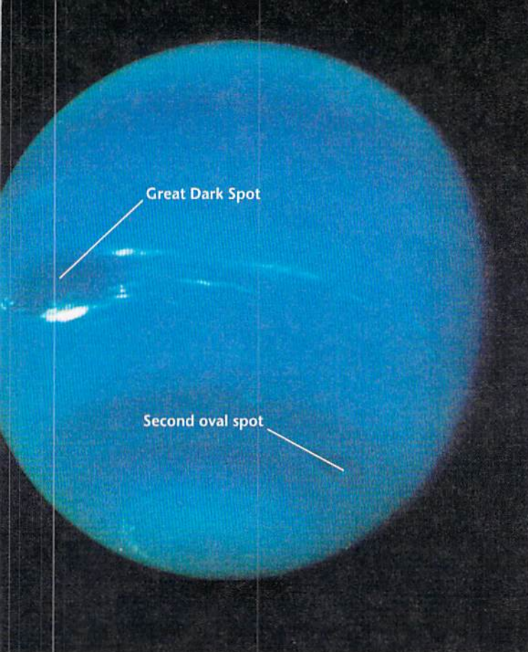
FIGURE 22.24 This image of Neptune shows the Great Dark Spot (left center). Also visible are bright cirruslike clouds that travel at high speeds around the planet. A second oval spot is at 54^\circ south latitude. (Courtesy of the Jet Propulsion Laboratory)
