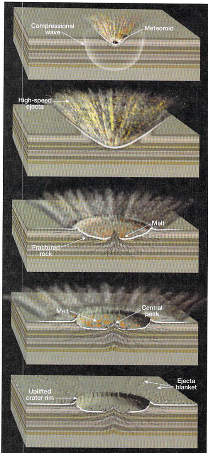
FIGURE 22.4 Formation of an impact crater. The energy of the rapidly moving meteoroid is transformed into heat energy and compressional waves. The rebound of the compressed rock causes debris to be ejected from the crater, and the heat melts some material, producing shock-melted glass. Small secondary craters are often formed by the material “splashed” from the impact crater. (After E. M. Shoemaker)
