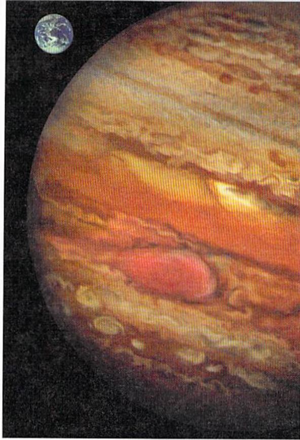
FIGURE 22.17 Artist's view of Jupiter with Great Red Spot visible in its southern hemisphere. Earth for scale.
