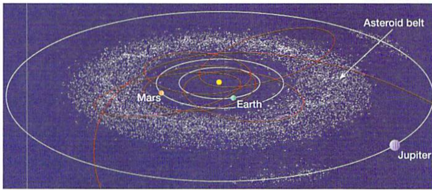
FIGURE 22.25 The orbits of most asteroids lie between Mars and Jupiter. Also shown are the orbits of a few known near-Earth asteroids. Perhaps a thousand or more asteroids have near-Earth orbits. Luckily, only a few dozen are thought to be larger than 1 kilometer in diameter.
