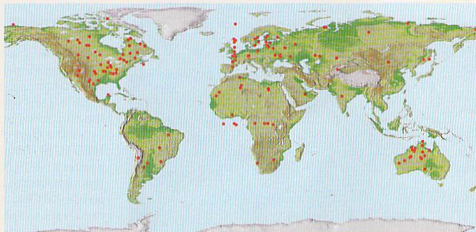
FIGURE 22.B World map of major impact structures. Others are being identified every year. (Data from Griffith Observatory)
