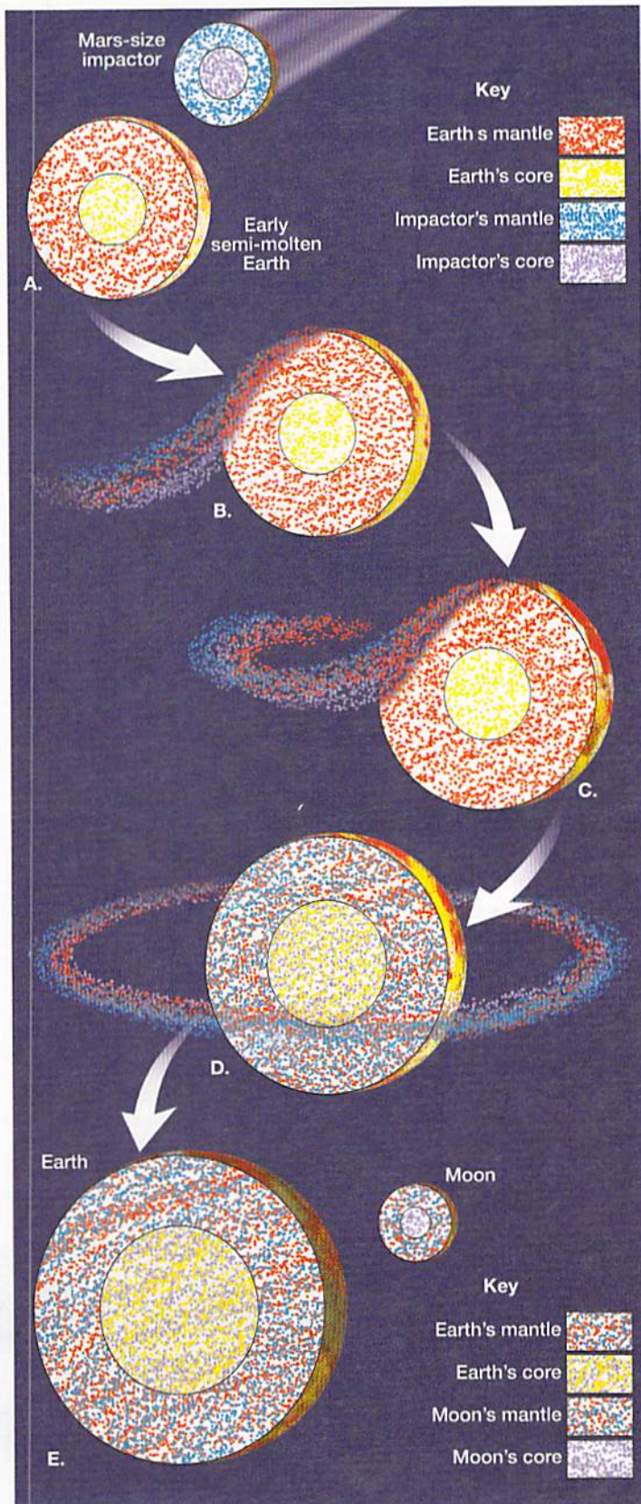
FIGURE 22.9 The formation of the Moon based on a scenario often called the impact theory. According to this model a protoplanet the size of Mars was involved in a glancing collision with a young semi-molten Earth. Most of the pieces of the protoplanet and splattered fragments of Earth coalesced in an orbit to form the Moon. Note that much of the impactor's core became part of Earth, leaving the Moon with a large rocky mantle and a comparatively small metallic core.
