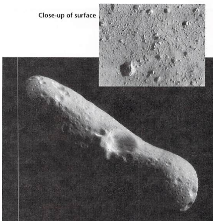
FIGURE 22.26 Image of asteroid Eros obtained by the NEAR-Shoemaker probe. Inset shows a closeup of Eros's barren, rocky surface. (Courtesy of HO, John Hopkins University Applied Physics Laboratory/AP Wide World Photos)
