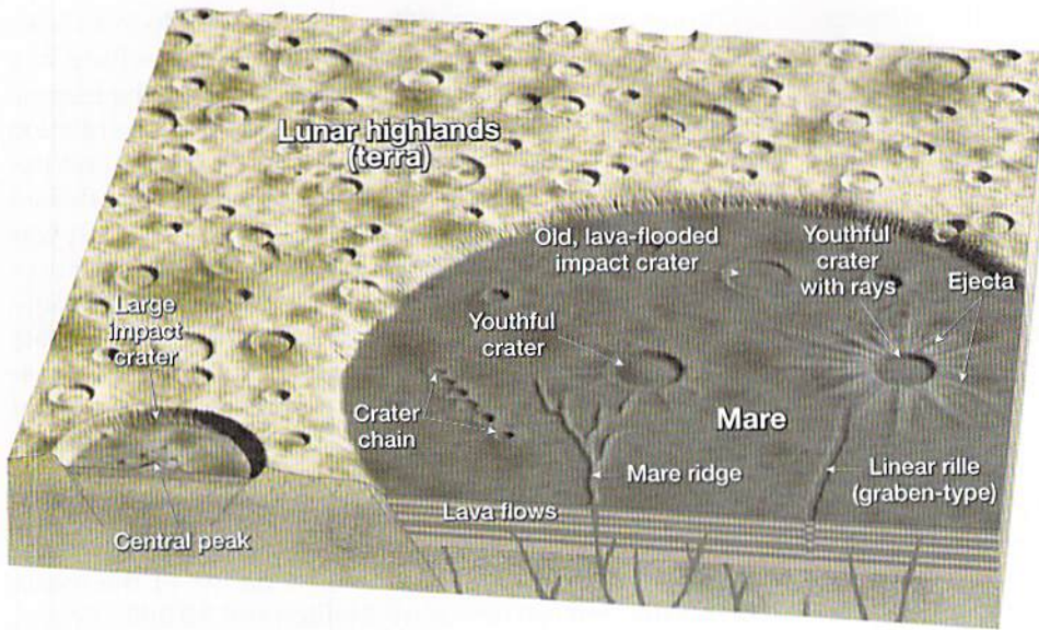
FIGURE 22.6 Block diagram illustrating the major topographic features on the lunar surface.
