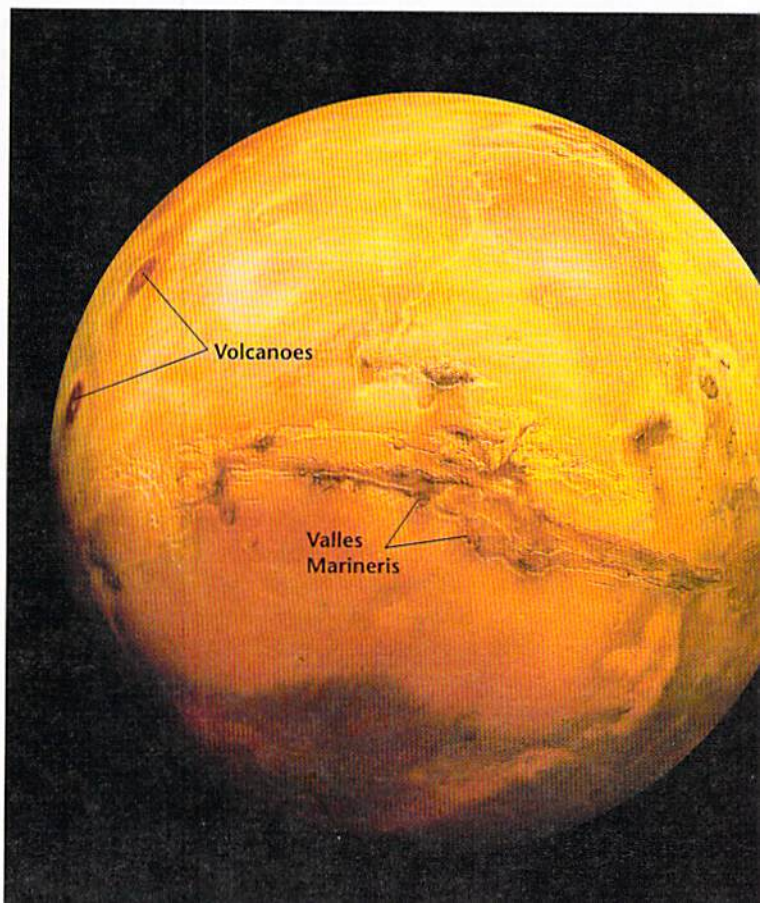
FIGURE 22.14 This image shows the entire Valles Marineris canyon system, more than 5,000 kilometers (3,000 miles) long and up to 8 kilometers (5 miles) deep. The dark spots on the left edge of the image are huge volcanoes, each about 25 kilometers high. (Courtesy of U.S. Geological Survey)
