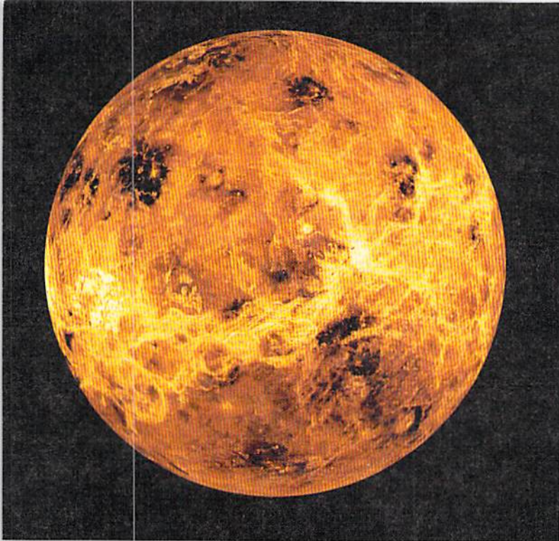
FIGURE 22.11 This global view of the surface of Venus is computer-generated. It resulted from two years of Magellan Project radar mapping. The bright, twisting features that cross the globe are highly fractured mountains and canyons of the eastern Aphrodite highland. (Courtesy of NASA/JPL)
