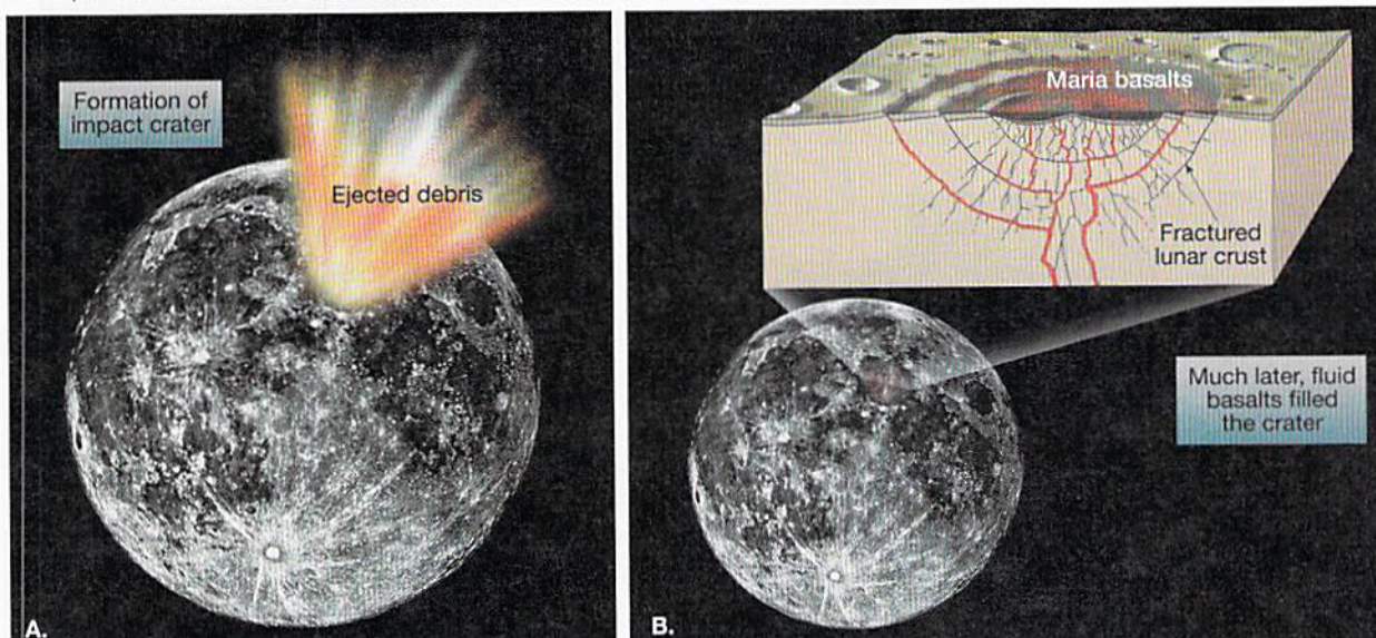
FIGURE 22.7 Formation of lunar maria. A. Impact of an asteroid-size mass produced a huge crater hundreds of kilometers in diameter and disturbed the lunar crust far beyond the crater. B. Filling of the impact area with fluid basalts, perhaps derived from partial melting deep within the lunar mantle.
