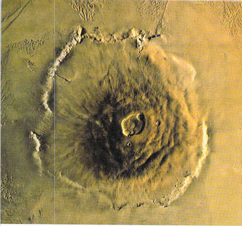
FIGURE 22.13 Image of Mons Olympus, an inactive shield volcano on Mars that covers an area about the size of the state of Ohio. (Courtesy of the U.S. Geological Survey)
