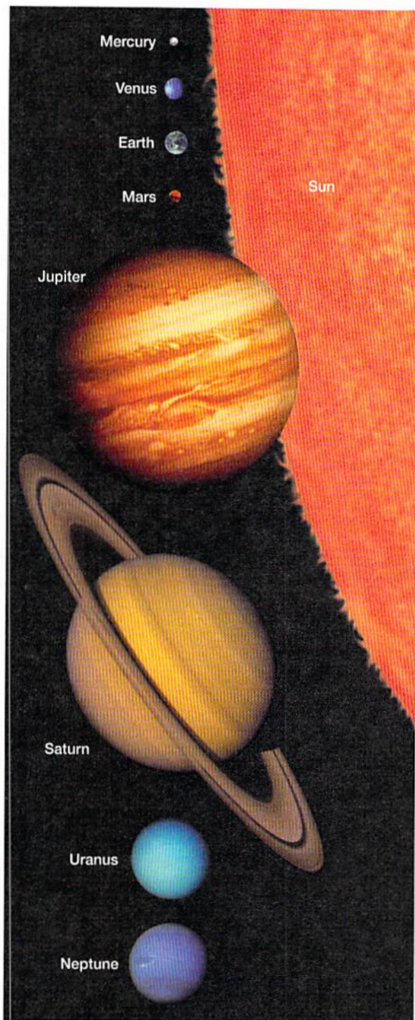
FIGURE 22.2 The planets drawn to scale.
