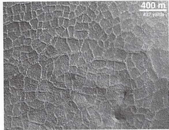
FIGURE 22.16 Polygonal patterned ground, shown here on Mars, is common in areas of permafrost in polar latitudes on Earth. (Courtesy of JPL/NASA)
