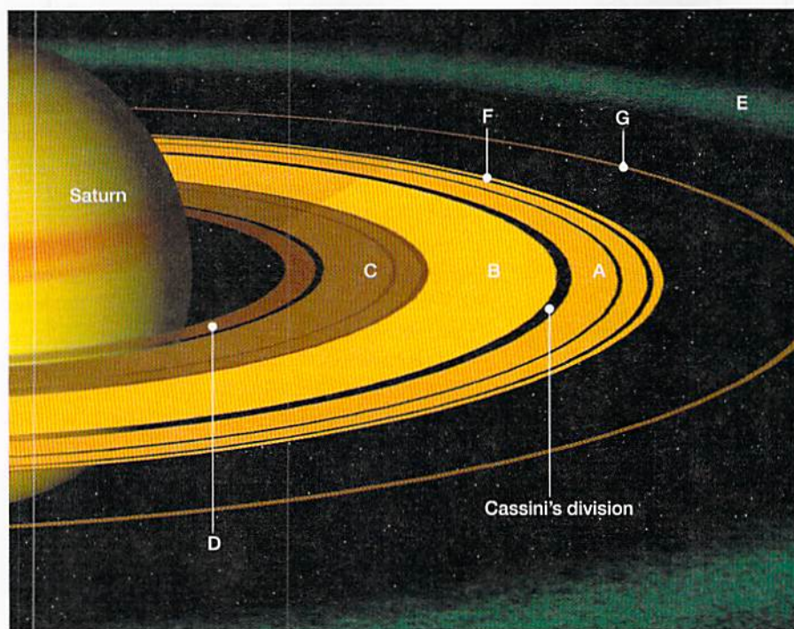
FIGURE 22.21 A view of the dramatic ring system of Saturn.
