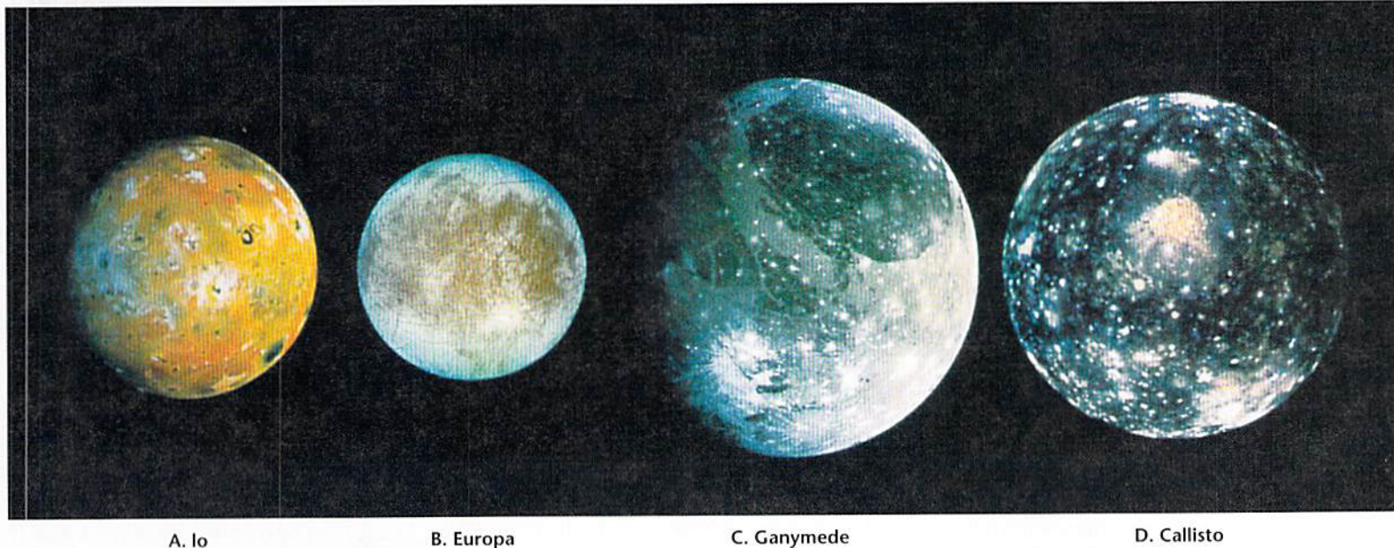
FIGURE 22.19 Jupiter's four largest moons (from left to right) are called the Galilean moons because they were discovered by Galileo. A. The innermost moon, Io, is one of only three volcanically active bodies in the solar system. B. Europa, smallest of the Galilean moons, has an icy surface that is criss-crossed by many linear features. C. Ganymede, the largest Jovian satellite, contains cratered areas, smooth regions, and areas covered by numerous parallel grooves. D. Callisto, the outermost of the Galilean satellites, is densely cratered, much like Earth's moon. (Courtesy of NASA/NGS Image Collection)
