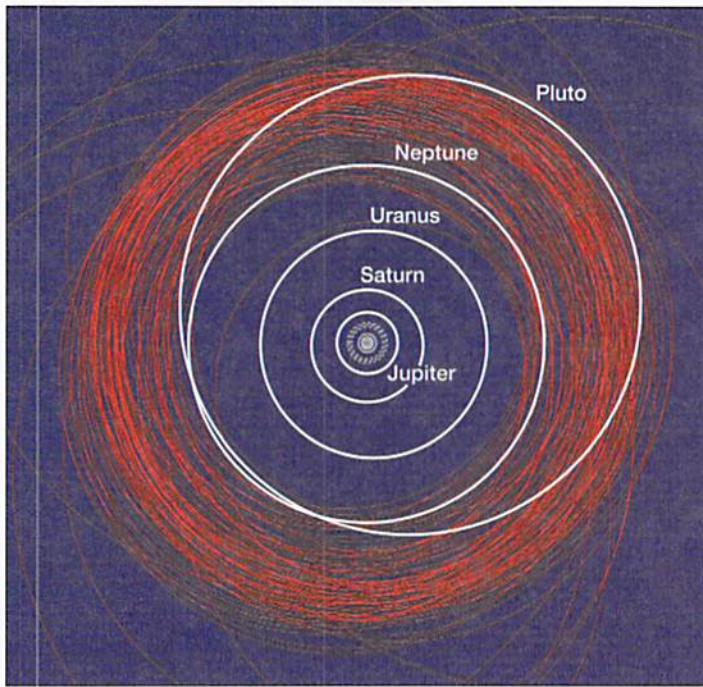
FIGURE 22.28 The orbits of some known Kuiper belt objects.
