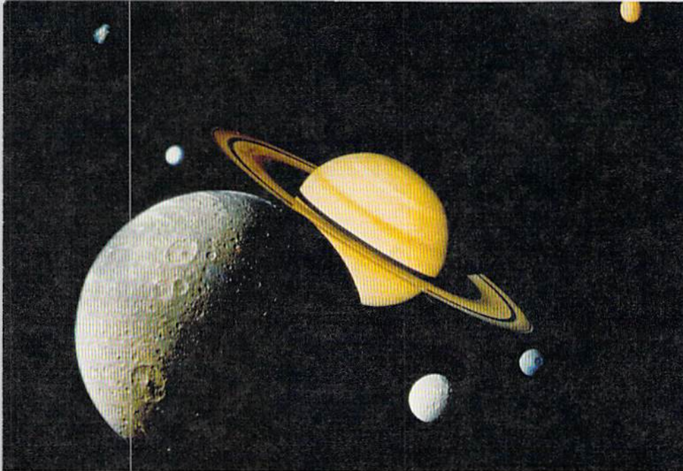
FIGURE 22.22 Montage of the Saturnian satellite system. The moon Dione is in foreground; Tethys and Mimas are at lower right; Enceladus and Rhea are off ring's left; and Titan is upper right. (Image courtesy of NASA)
