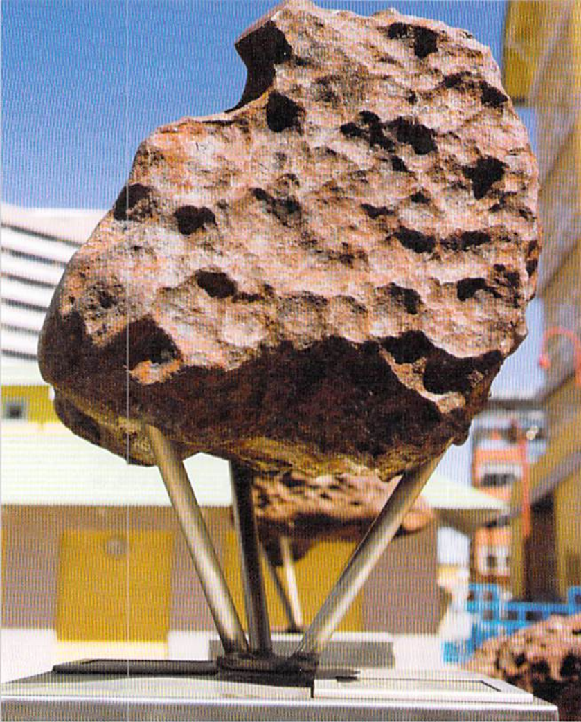
FIGURE 22.29 Iron meteorite found in Namibia, a country in southwestern Africa. (Photo by Neil Setchfield/Alamy)
