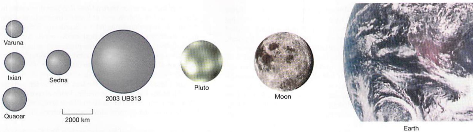
FIGURE 22.31 Pluto, a dwarf planet compared to some large Kuiper belt objects. The Earth–Moon system added for scale. (Courtesy of NASA)
