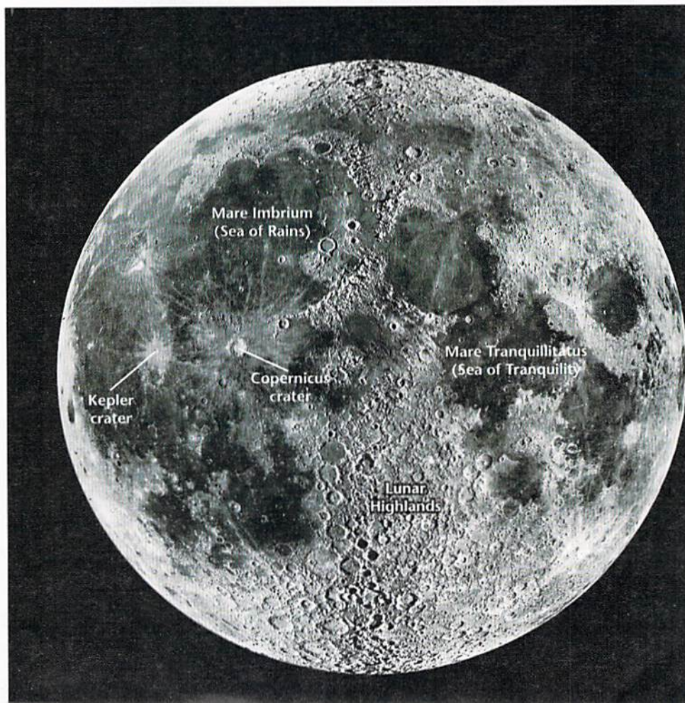
FIGURE 22.3 Telescopic view from Earth of the lunar surface. The major features are the dark “seas” (maria) and the light highly cratered lunar highlands (terrae). (UCO/Lick Observatory Image)
