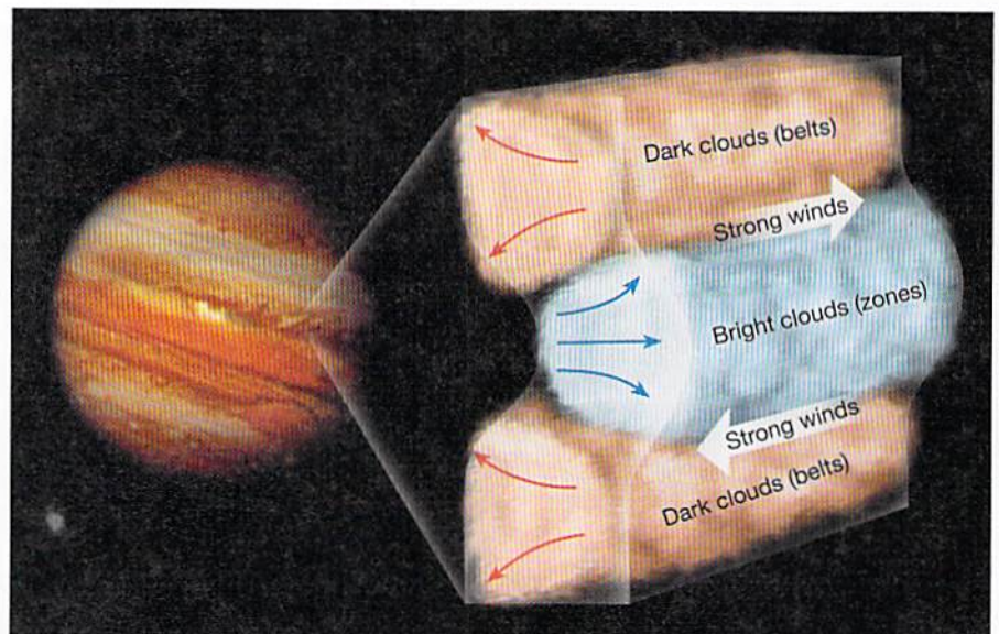
FIGURE 22.18 The structure of Jupiter's atmosphere. The areas of light clouds (zones) are regions where gases are ascending and cooling. Sinking dominates the flow in the darker cloud layers (belts). This convective circulation, along with the rapid rotation of the planet, generates the high-speed winds observed between the belts and zones.
